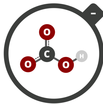
HYDROGEN CARBONATE
