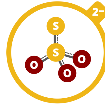
THIOSULFATE
