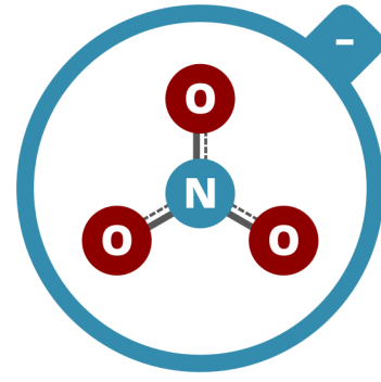
NITRATE
