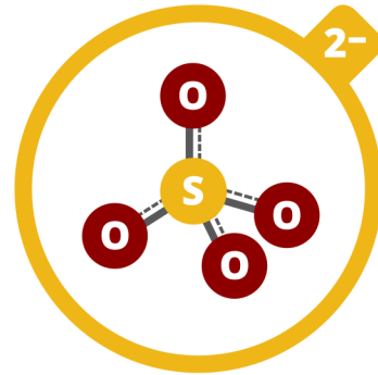
SULFATE
