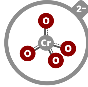
CHROMATE
