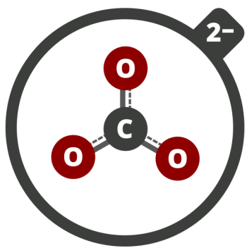
CARBONATE
