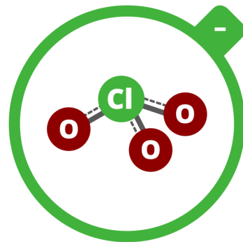
CHLORATE
