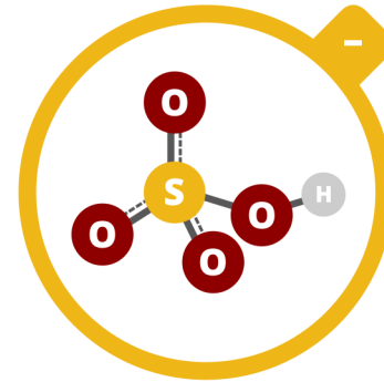
HYDROGEN SULFATE
