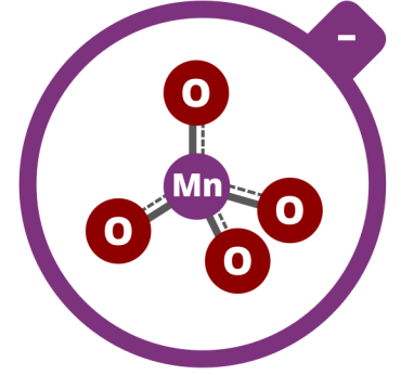
PERMANGANATE
