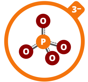
PHOSPHATE
